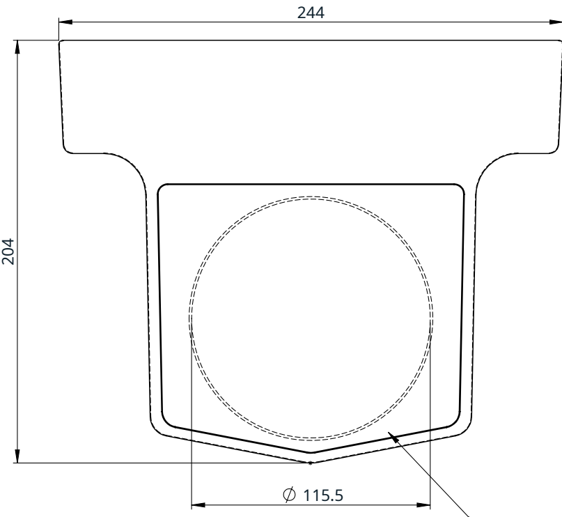
MALE END CAP
