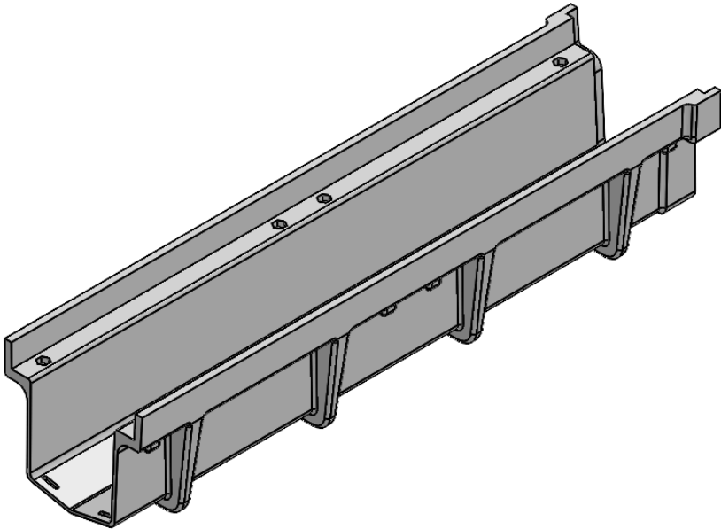
ISOMETRIC VIEW
