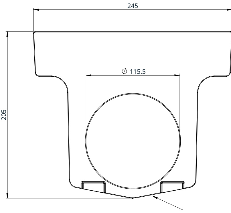
FEMALE END CAP
