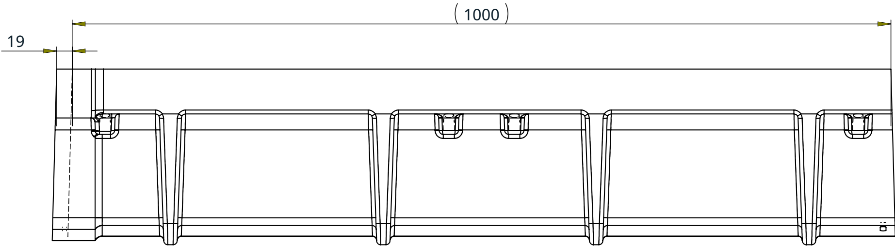
SIDE VIEW
